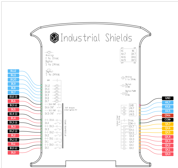
M-Duino Analog/Digital Zone Pinout Zone B: X = 0 Zone C: X = 1 Zone D: X = 2 Legend: ● Ground ● Analog ● PWM ● Digital ● Power ● Input ○ Output ○ Input/Output
