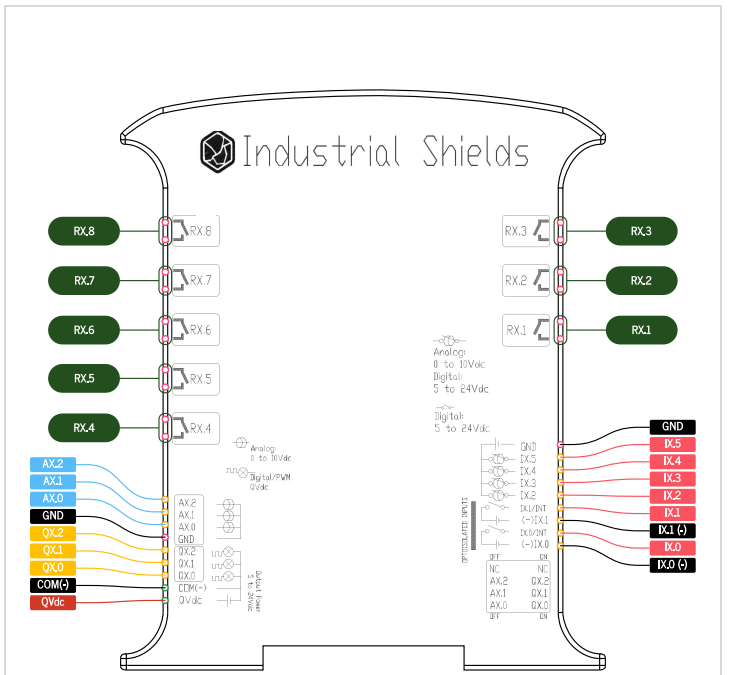
M-Duino Relay Zone Pinout Zone B: X = 0 Zone C: X = 1 Zone D: X = 2 Legend: ● Ground ● Analog ● PWM ● Digital ● Power ● Input ○ Output ○ Input/Output ■ Relay
